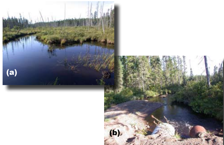
Figure 1.19—Roadfill effects on flood-plain hydrology—Minnesota. (a) Meandering channel with half-mile-wide flood plain remains backwatered for several weeks during snowmelt runoff, and sediment deposition extends for thousands of feet upstream. High water tables have killed the flood-plain trees. (b) Downstream view from same point as (a).
