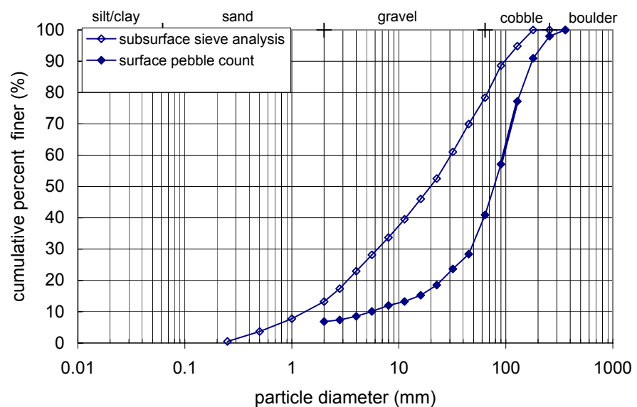
Figure 5.6—Surface armor and subsurface particle size distribution curves for the South Fork Cache la Poudre River (data from Bunte 2004). The surface armor was characterized by a pebble count. The subsurface was bulk sampled and sieved. Although the subsurface has a higher content of fines, it also includes the full range of coarser sizes found in the surface armor.
