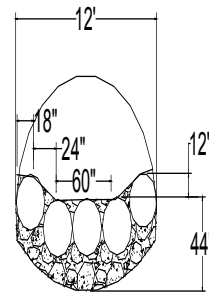
Step-pool step boulder details x-section AA'.
