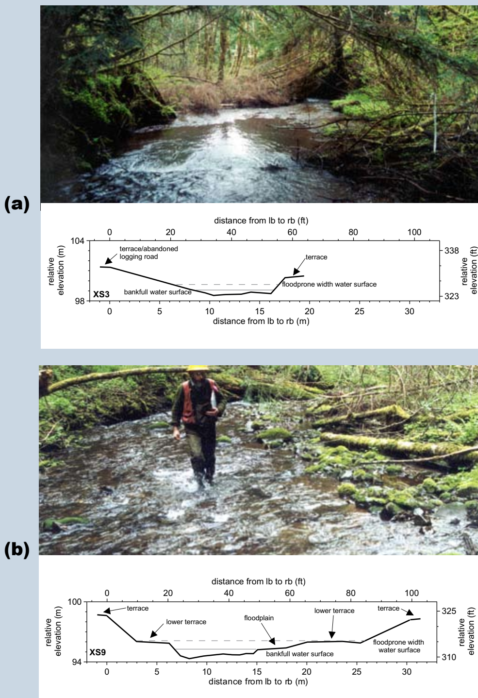
Figure 5.10—Newbury Creek cross-section profiles and photos. (Cross-sections are plotted looking downstream and their locations are shown in figure 5.9.) (a) Looking downstream toward cross sections 3 and 4 (photo taken between cross section 2 and cross section 3). Two log weirs are visible. In the background a bedrock outcrop is exposed on the right bank of the channel. (b) Looking downstream at cross section 9.
