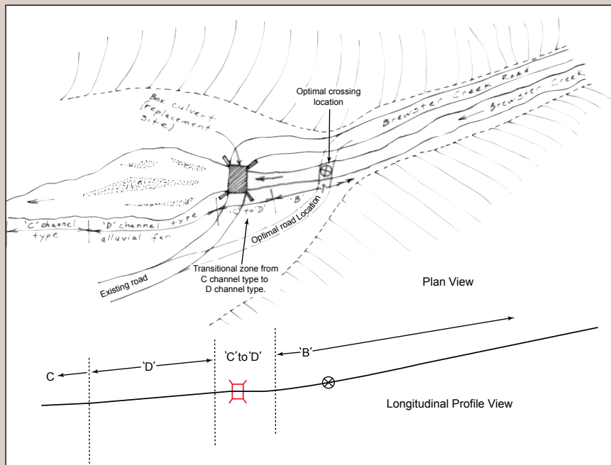
Figure 4.7—Brewster Creek crossing plan-view sketch. Original drawing by Traci Sylte.
