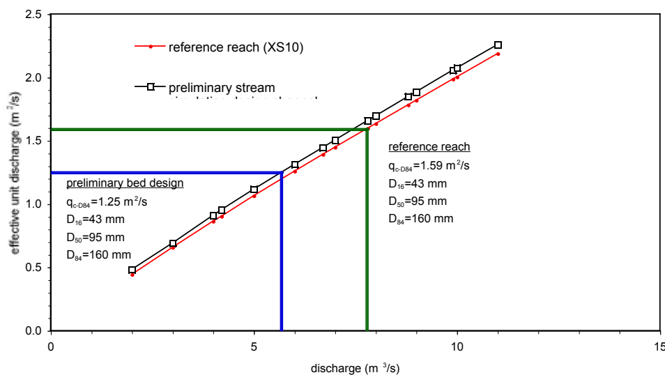
Figure E.8—Plot of unit discharge versus discharge showing when the D_{84} particle is mobilized in the reference-reach channel and the preliminary stream-simulation design channel. To achieve similar D_{84} particle mobility in the stream simulation design channel at the same flow as the reference-reach channel, the D_{16} , D_{50} , and D_{84} particle sizes were increased in size by 17.5 percent to 50 mm, 112 mm, and 188 mm, respectively.
