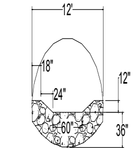
Infill pattern for streambed-simulation material.
