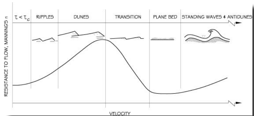
Figure A.14—Depending on flow intensity, bed structures such as ripples, dunes, and antidunes can form in sand bed channels, dramatically changing channel roughness. Redrawn after Simons, Li & Associates 1982.
